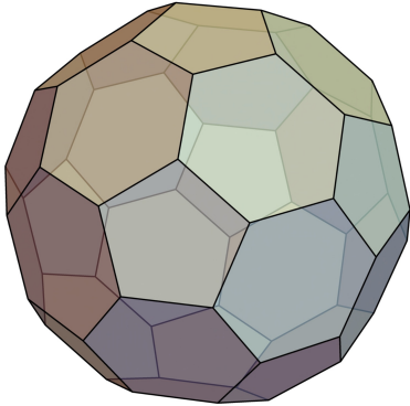
TRUNCATED ICOSAHEDRON
