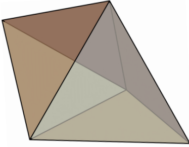
TRIANGULAR DIPYRAMID
