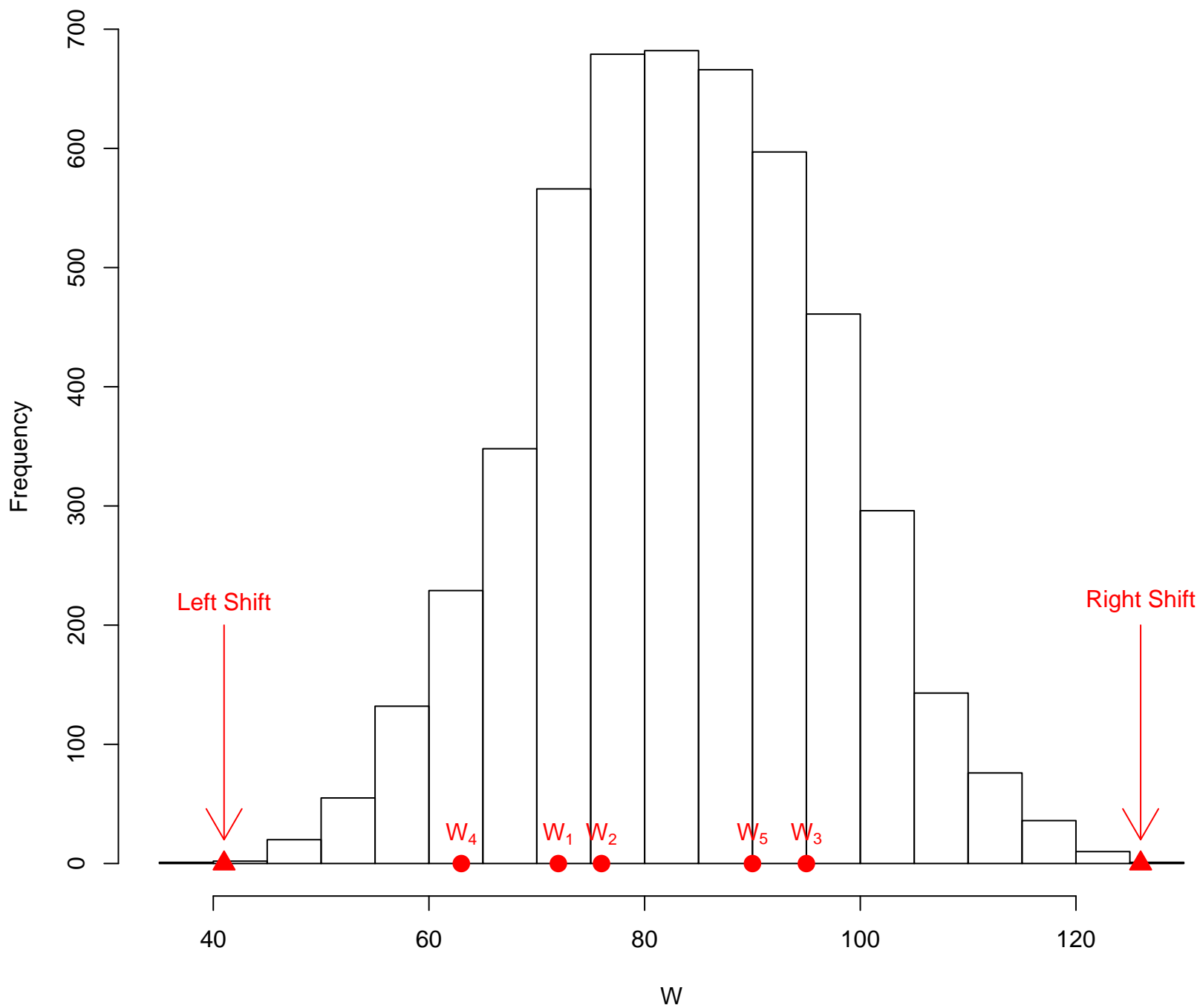
Histogram of W for 5000 simulated data sets with equal medians
